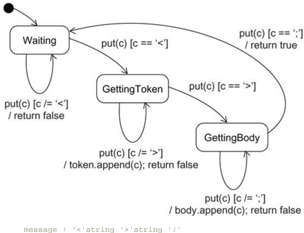
Figure 24-2 Modeling Reactive Objects
