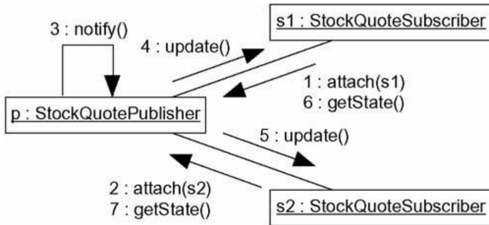
Figure 15-7 Flow of Control by Organization
