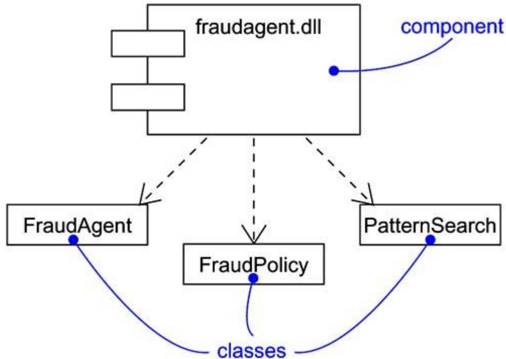
Figure 25-3 Components and Classes
